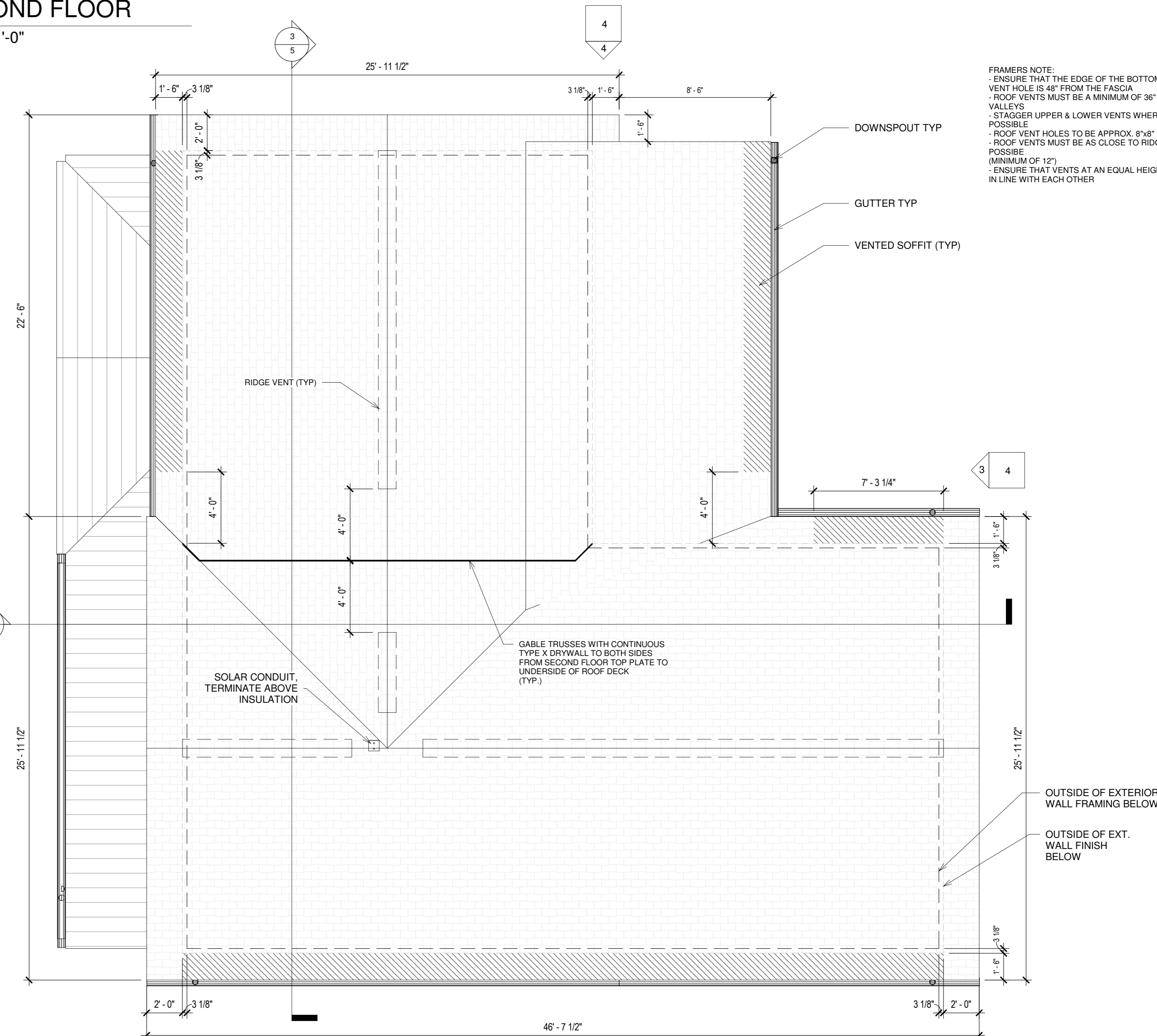
4 ROOF PLAN 1/4" = 1'-0" ROOF AREA: 2353 SQ FT
