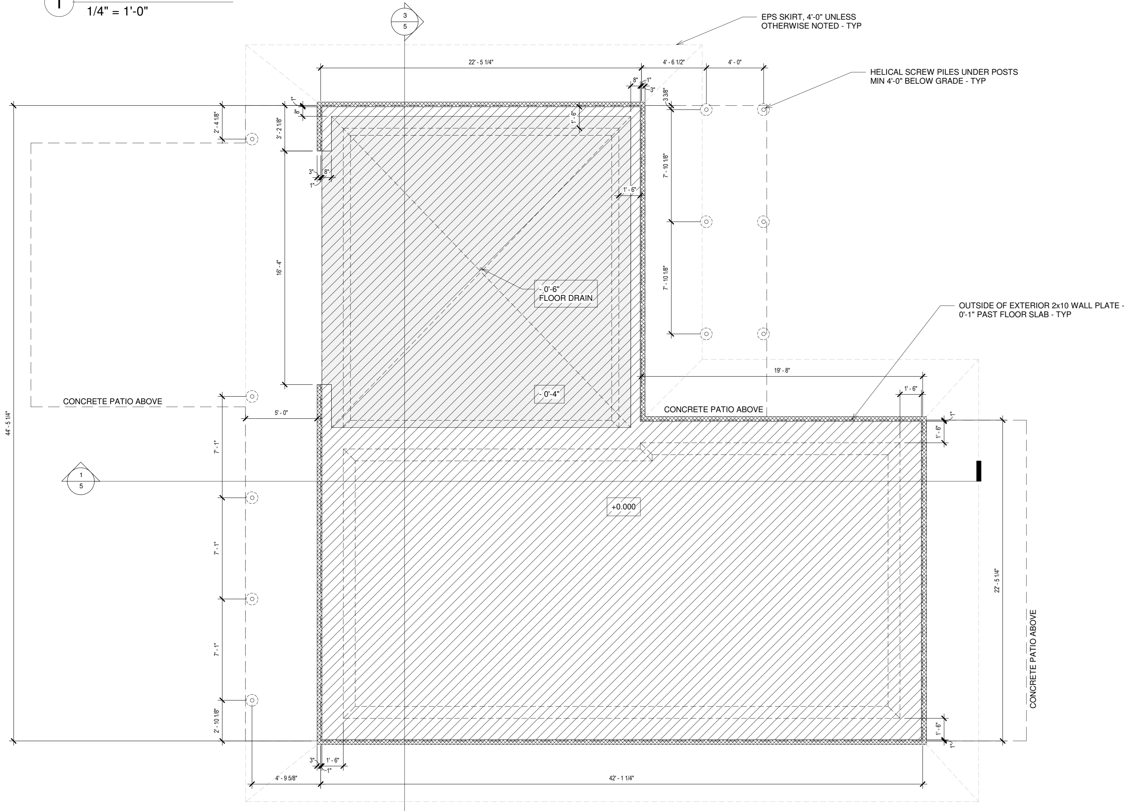
3 FOUNDATION PLAN 1/4" = 1'-0"
