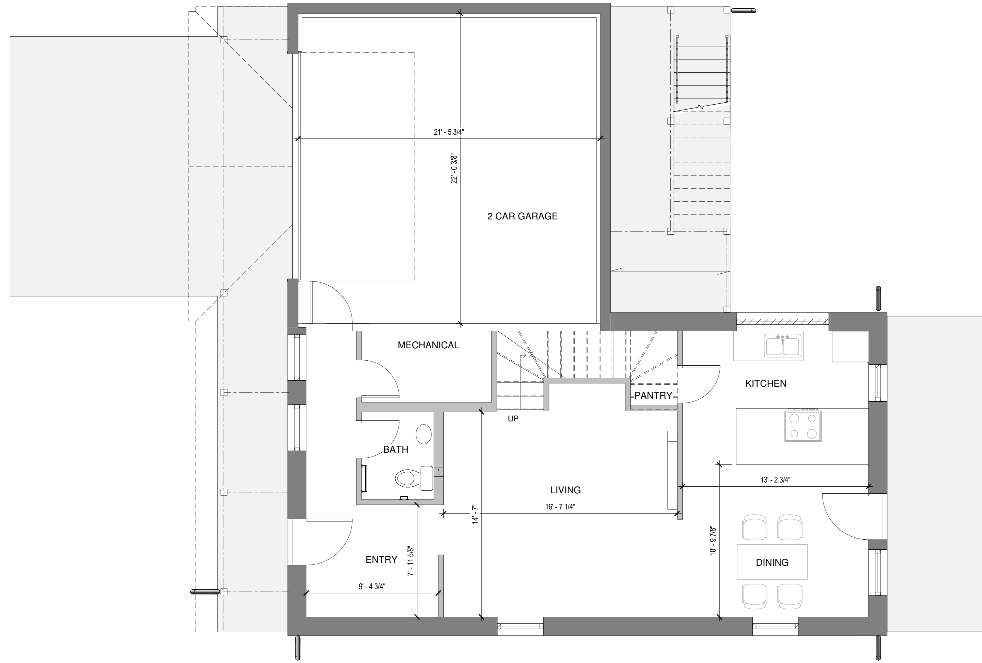
1 MAIN FLOOR 1/4" = 1'-0"
