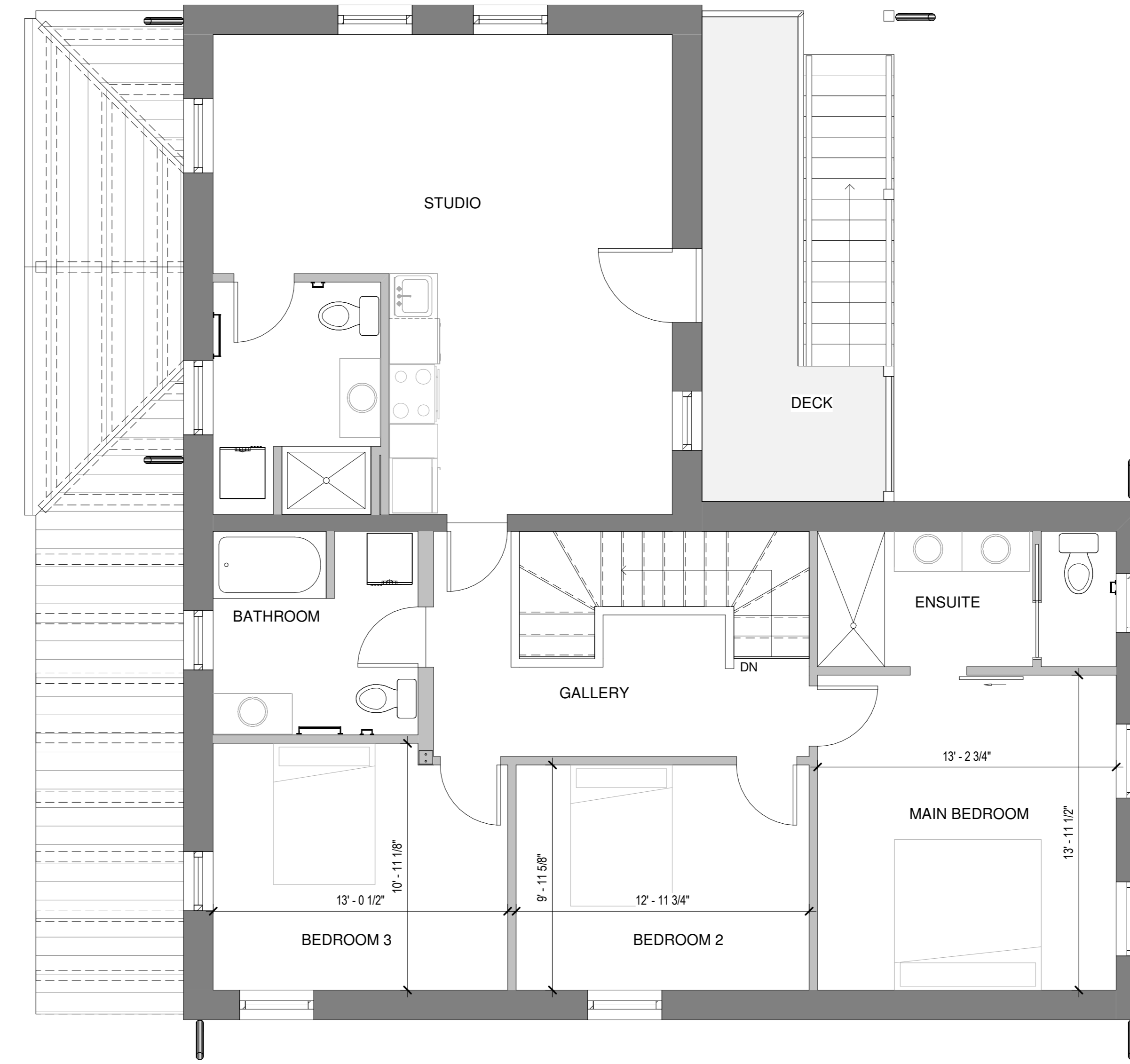
2 SECOND FLOOR 1/4" = 1'-0"
